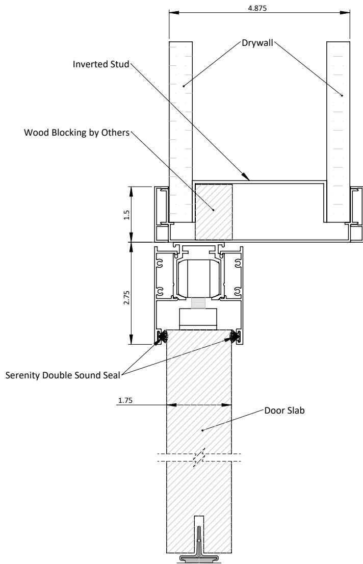
EvenView w/ Cased Open Mount
