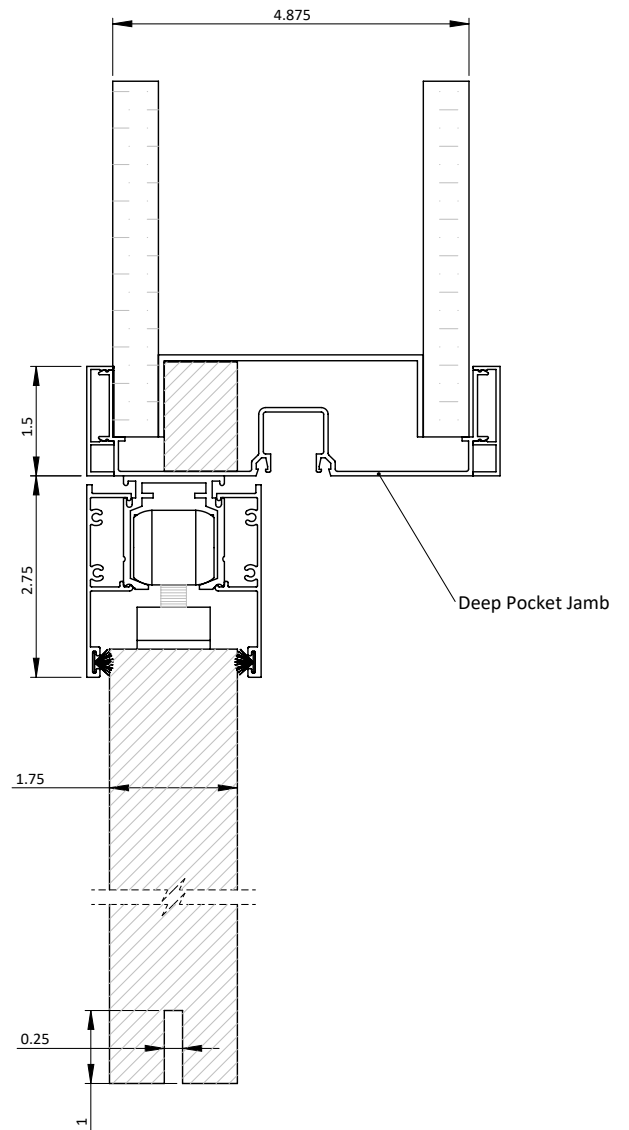
EvenView w/ Pocket Jamb Mount
