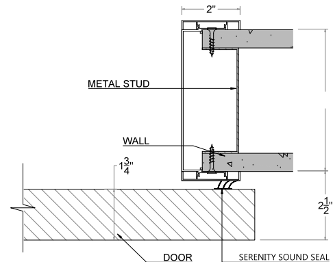
DETAIL 03 SCALE 4"=1'-0"
