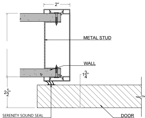
DETAIL 02 SCALE 4"=1'-0"
