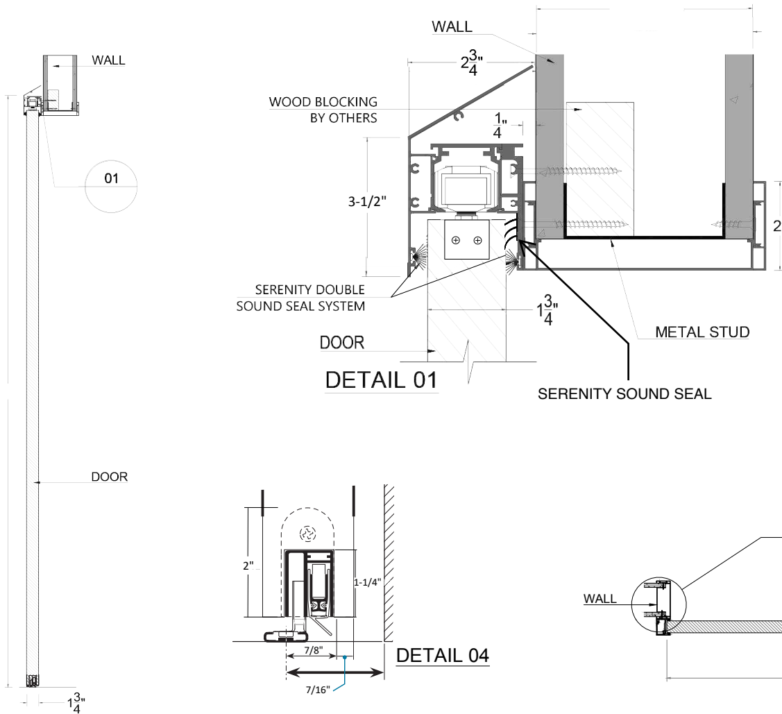
VIEW B - B SCALE 3/4"=1'-0"
