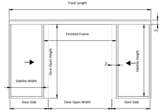
SyncSlide w/ Sidelite
