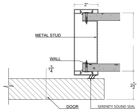
DETAIL 03 SCALE 4"=1'-0"
