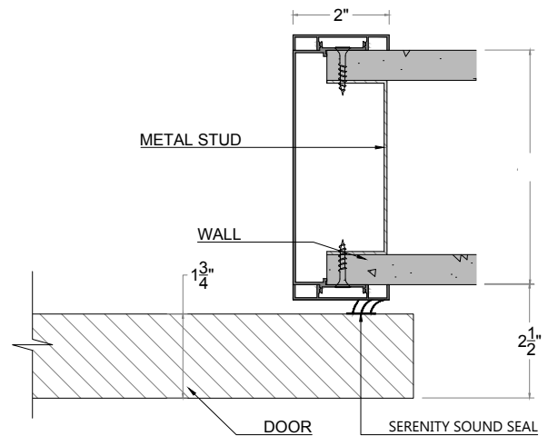
DETAIL 03 SCALE 4"=1'-0"
