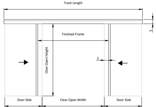
SyncSlide - No Sidelite
