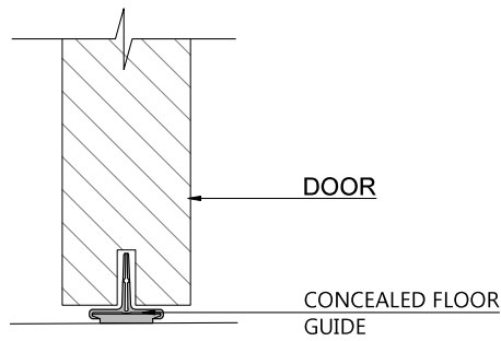
DETAIL 04 SCALE 4"=1'-0"
