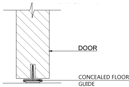
DETAIL 04 SCALE 4"=1'-0"
