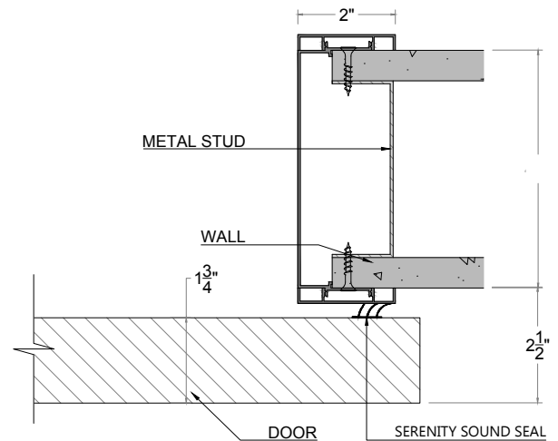
DETAIL 03 SCALE 4"=1'-0"
