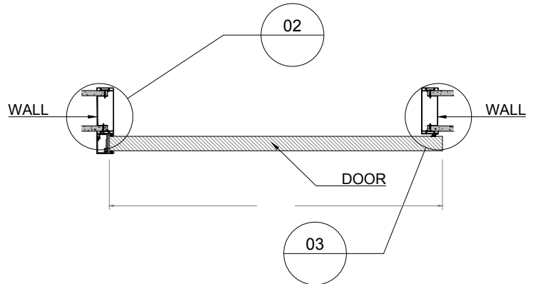
VIEW B - B SCALE 3/4"=1'-0"
