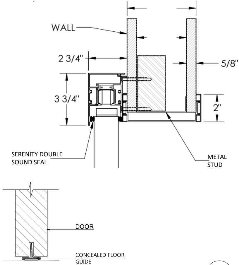
DETAIL 04 SCALE 4"=1'-0"
