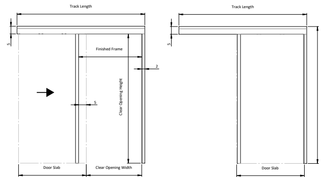
SecureSlide with Sloped Valance
