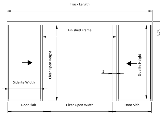
SyncSlide w/ Sidelite
