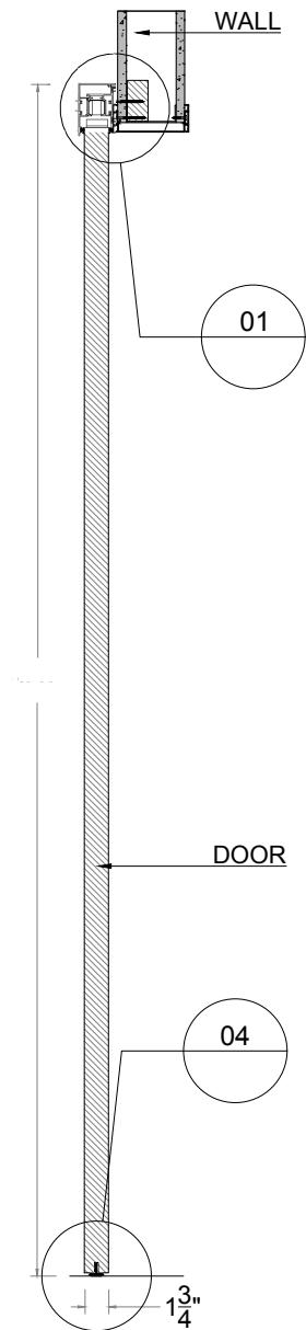
VIEW A - A SCALE 3/4"=1'-0"
