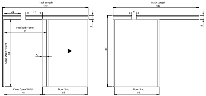
MedLift Slide with Sloped Valance
