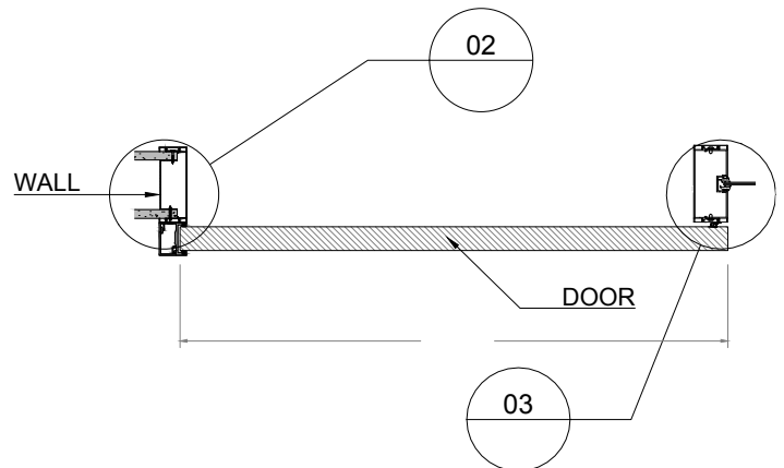
VIEW B - B SCALE 3/4"=1'-0"
