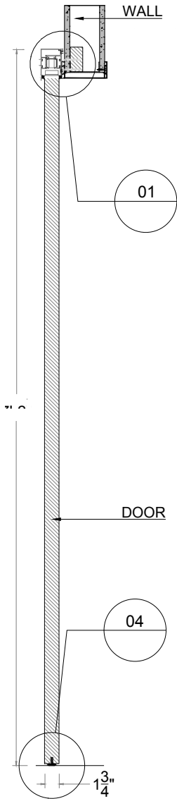
VIEW A - A SCALE 3/4"=1'-0"
