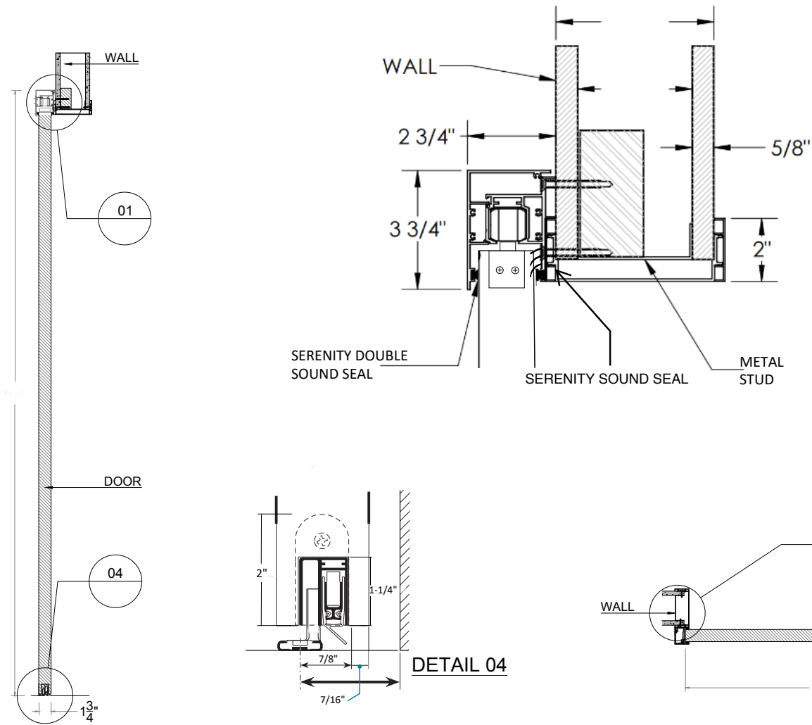
VIEW A - A SCALE 3/4"=1'-0"
