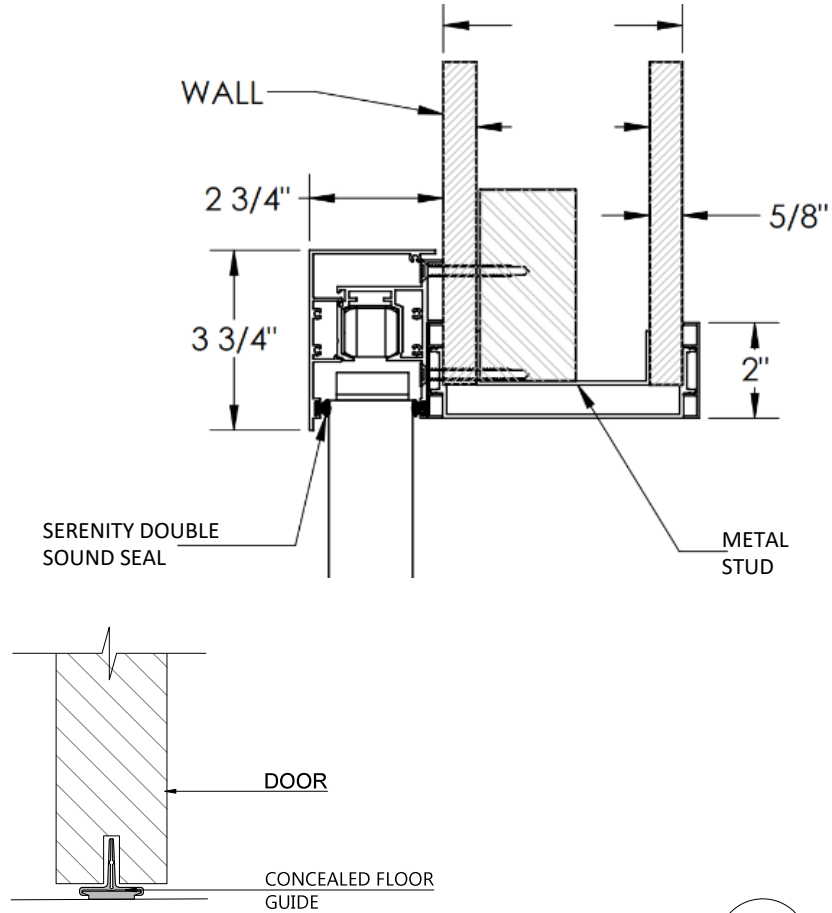
DETAIL 04 SCALE 4"=1'-0"
