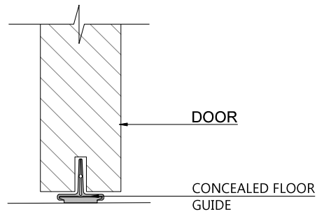
DETAIL 04 SCALE 4"=1'-0"
