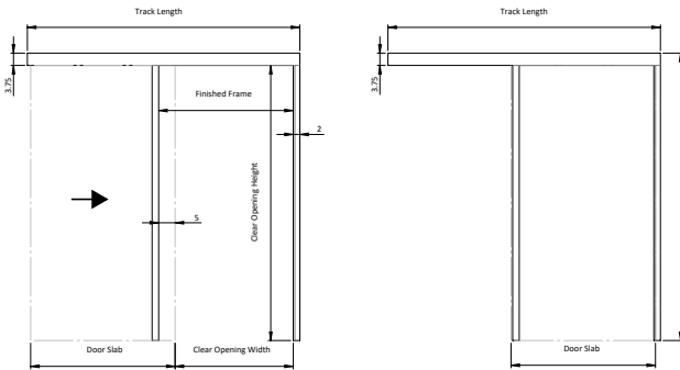
MedSlide with Squared Valance
