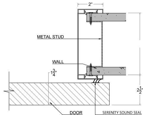
DETAIL 03 SCALE 4"=1'-0"
