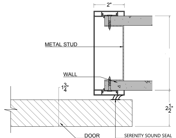
DETAIL 03 SCALE 4"=1'-0"
