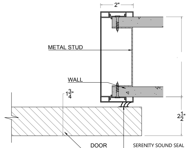
DETAIL 03 SCALE 4"=1'-0"
