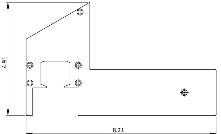
MedLift End Cap for Sloped Valance
