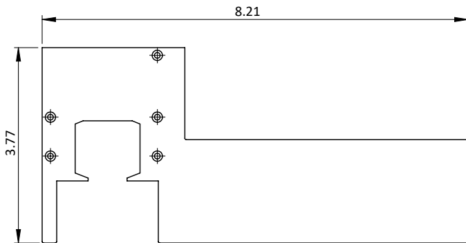
MedLift End Cap for Squared Valance
