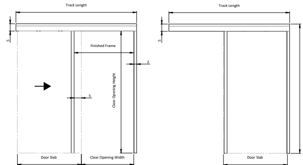
MedSlide with Sloped Valance
