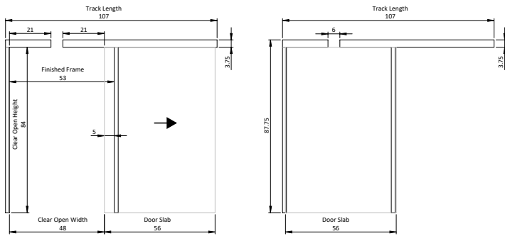
MedLift Slide with Squared Valance
