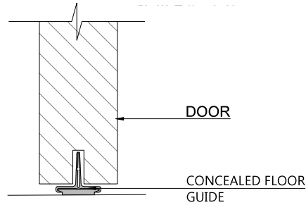
DETAIL 04 SCALE 4"=1'-0"
