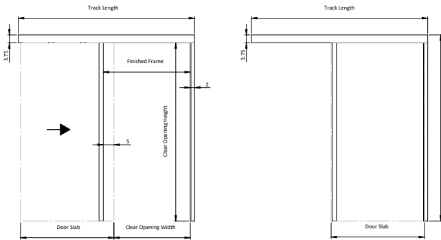
SmokeSlide with Squared Valance
