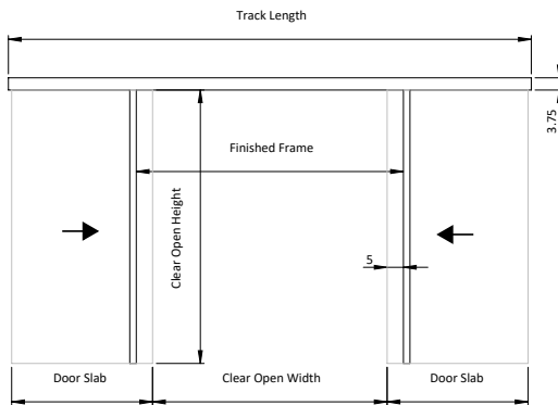
SyncSlide - No Sidelite
