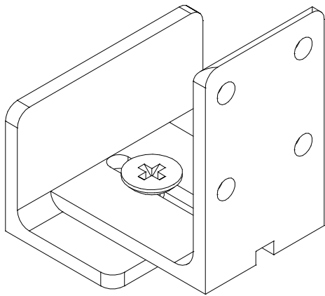
PART - 3D VIEW COUPLED SCALE 1'-0"=1'-0"
