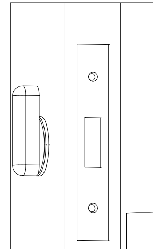
12" BACK TO BACK LADDER PULL SCALE 2"=1'-0"
