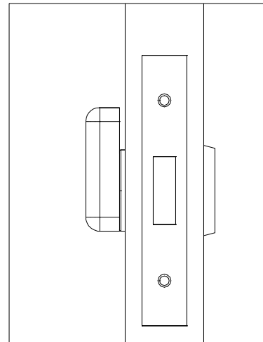
SMALL MORTISE LOCK SCALE 4"=1'-0"
